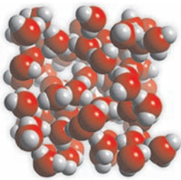
Water Molecules
